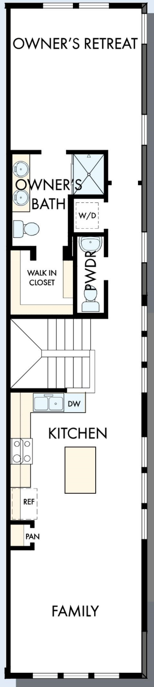
SECOND FLOOR
