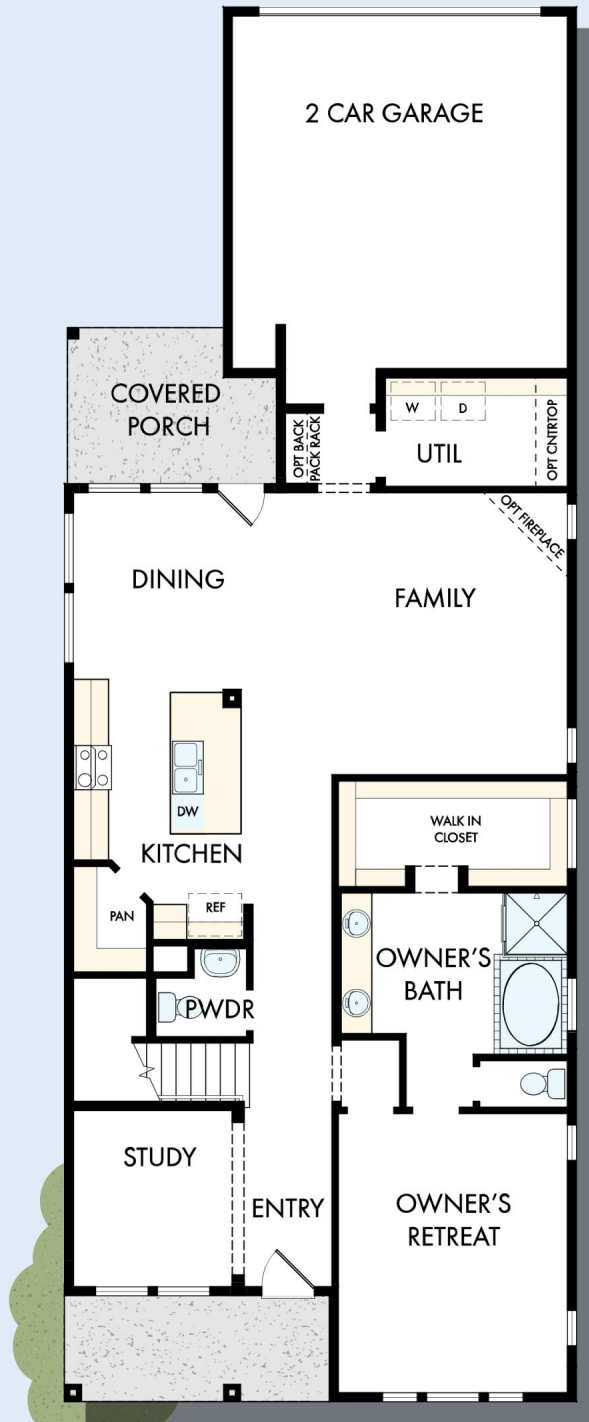
FIRST FLOOR
