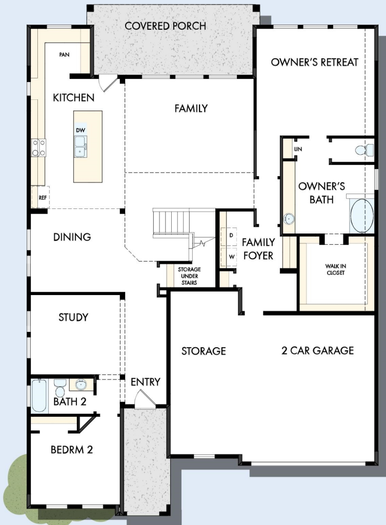
FIRST FLOOR
