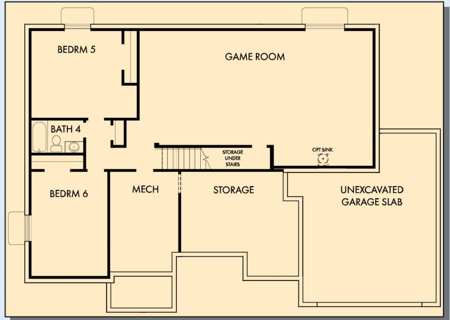
OPTIONAL GAME ROOM WITH BEDROOM 5, 6 AND BATH 4 AT BASEMENT
