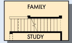
OPTIONAL FINISHED BASEMENT STAIRS WITH UNFINISHED BASEMENT
