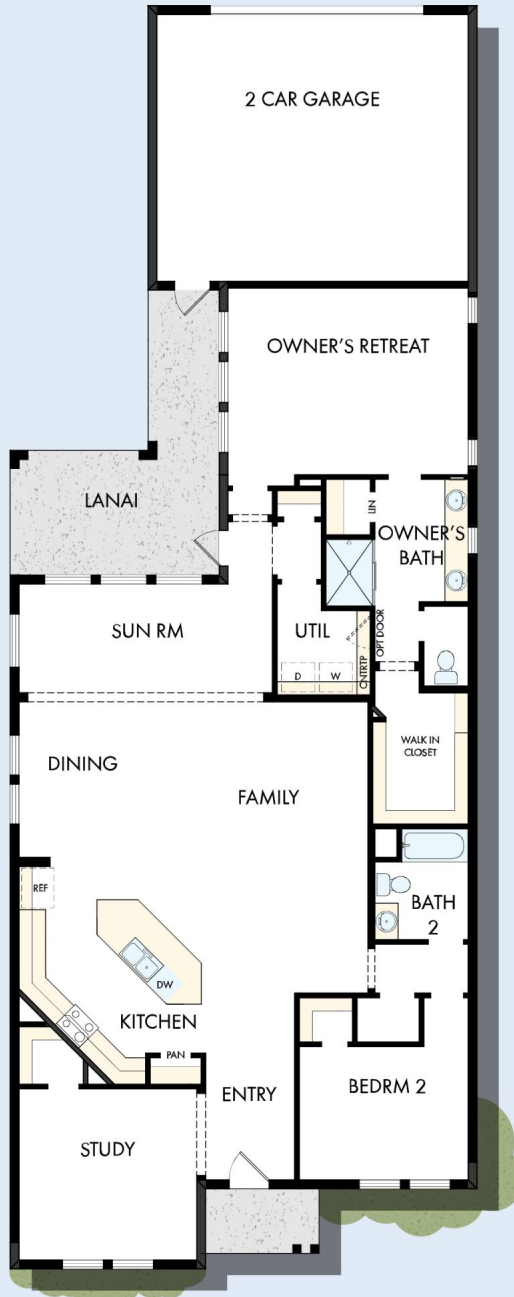
OPTIONAL SLIDE IN TUB WITH SEPARATE SHOWER AT OWNER'S BATH
