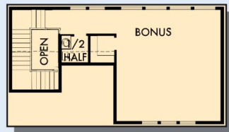
OPTIONAL SECOND FLOOR BONUS WITH HALF BATH
