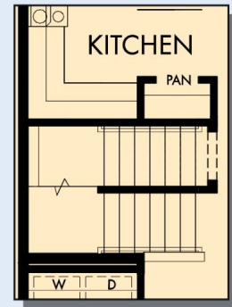
FIRST FLOOR WITH OPTIONAL FINISHED BASEMENT STAIRS
