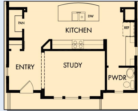
OPTIONAL ALTERNATE POWDER BATH AND PANTRY
