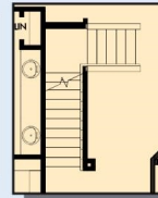
FIRST FLOOR WITH OPTIONAL FINISHED BASEMENT STAIRS
