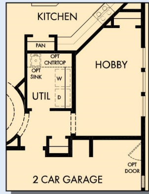
OPTIONAL HOBBY AT GARAGE
