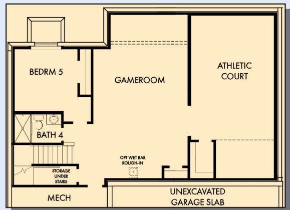
OPTIONAL GAMEROOM, BEDROOM 5, BATH 4 AND ATHLETIC COURT AT BASEMENT
